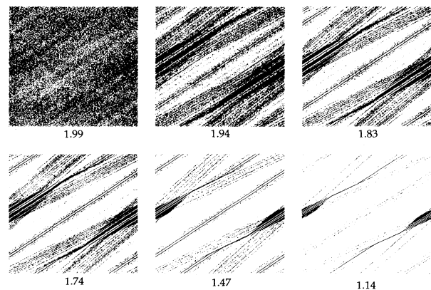
FIG. 6. Point distributions generated by iterating the map XYYPYX , where the values of the information dimension D_I , ranging downward from 1.99 to 1.14, are indicated on the distributions. The corresponding \Delta m values are 0.01, 0.05, 1/12, 0.10, 0.15, and 0.17.
